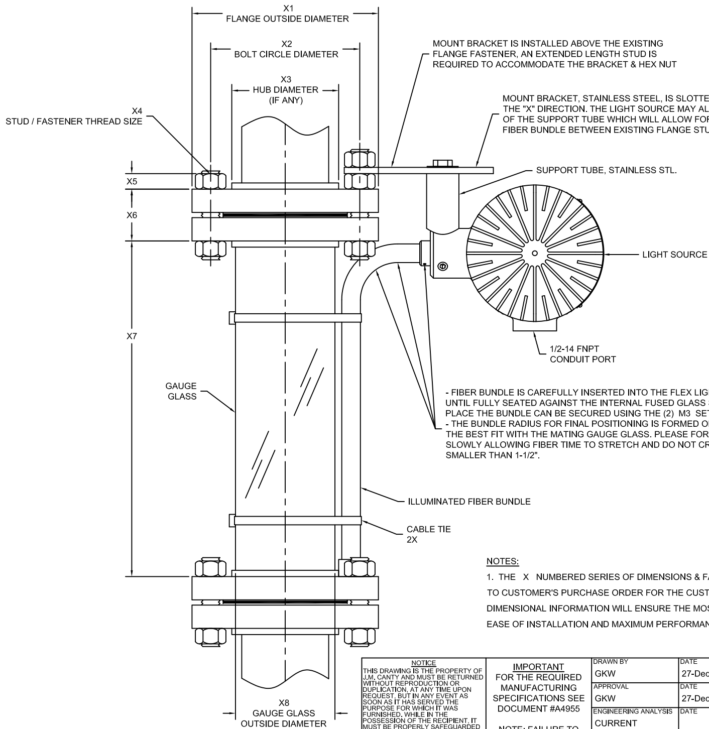
SIDE VIEW OF TYPICAL GAUGE LIGHT ASSEMBLY
