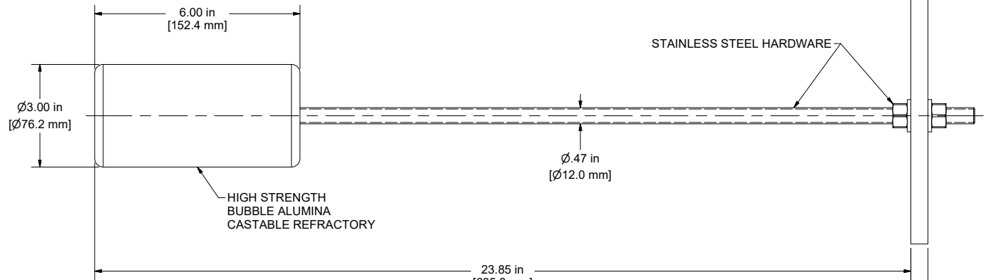
RIGHT SIDE VIEW SCALE .50 : 1
